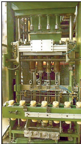
2000 OMP SRL PRESS PILLAR CANDLE MACHINE
